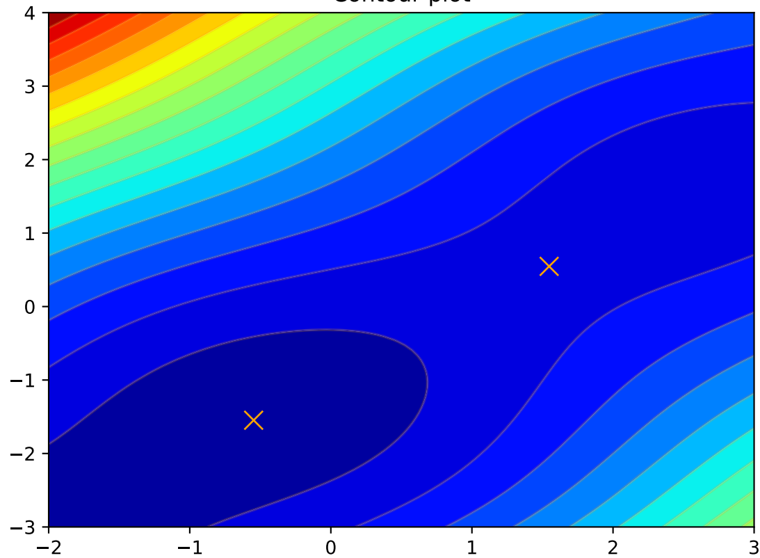
Contour plot
