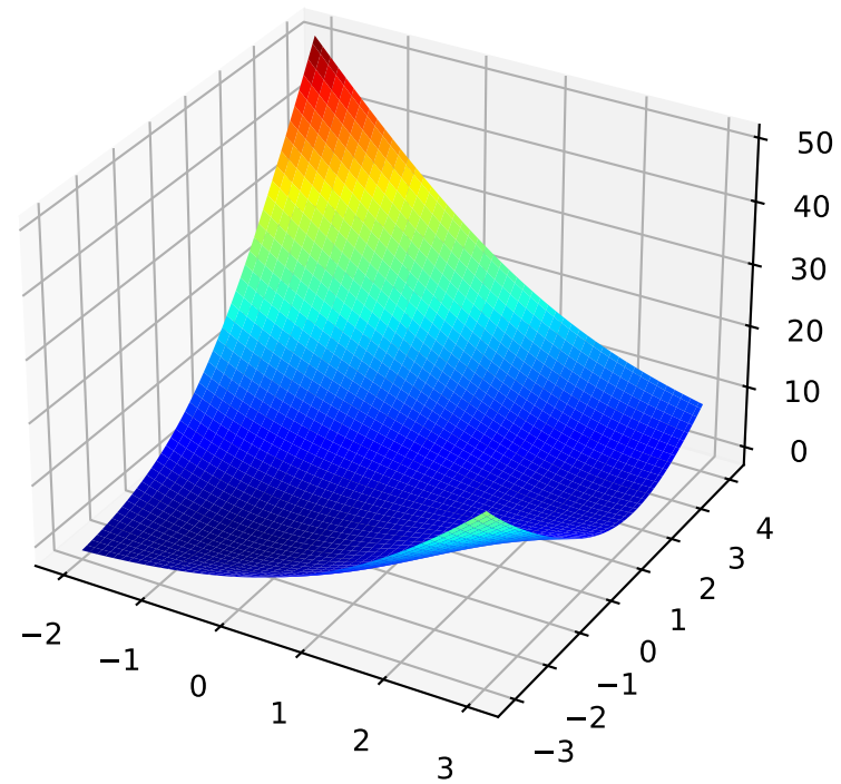
Surface plot
